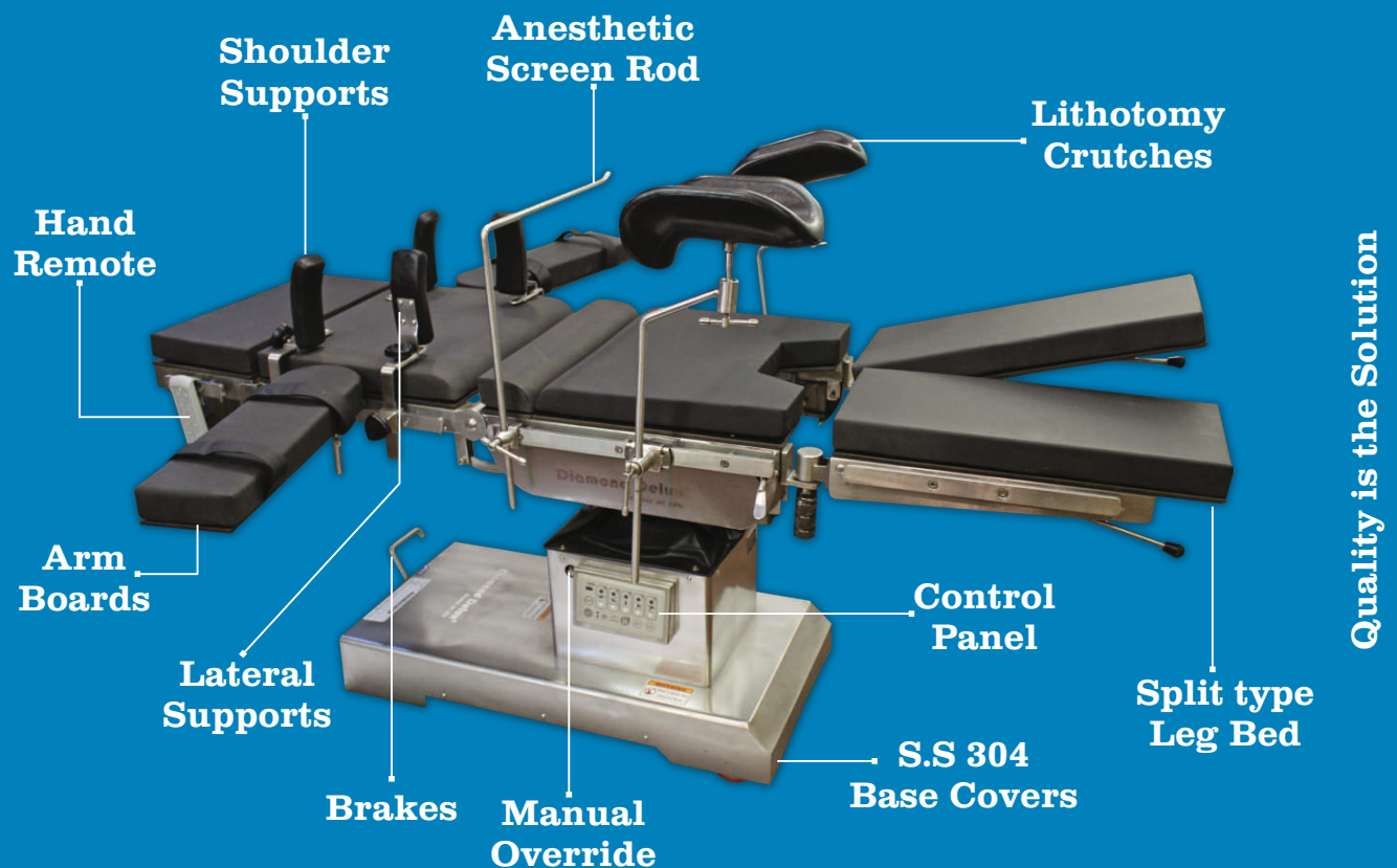
Electric Surgical table with Manual Override
